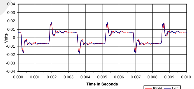
300 Hz Square Wave
